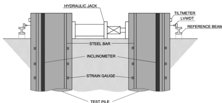
Fig. 26 Schematic of monitoring for lateral pile load test
