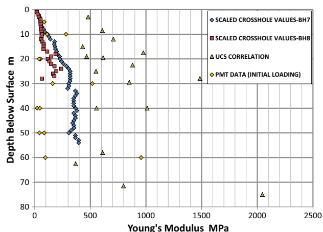
Fig. 31 Young's modulus values derived from various sources
