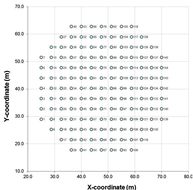
Fig. 32 Pile layout for tower
