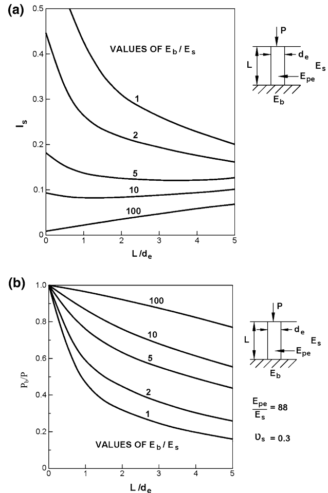
Fig. 2 a Settlement of equivalent pier in soil layer [57]. S = P \cdot I_s / d_e \cdot E_s . b Proportion of base load for equivalent pier [57]
