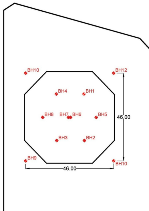
Fig. 29 Site plan and borehole locations
