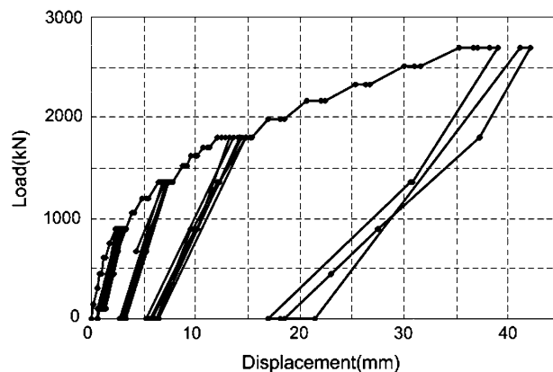
Fig. 27 Load versus displacement curve TP5
