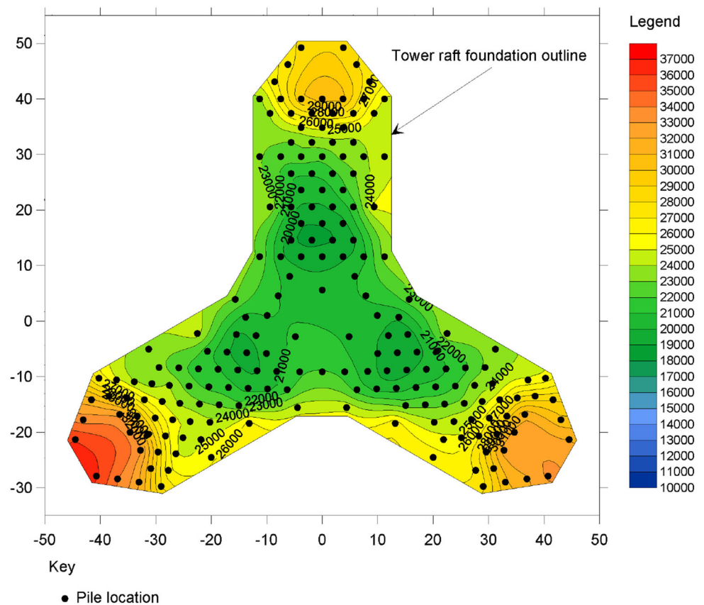
Fig. 12 Contours of maximum axial load
