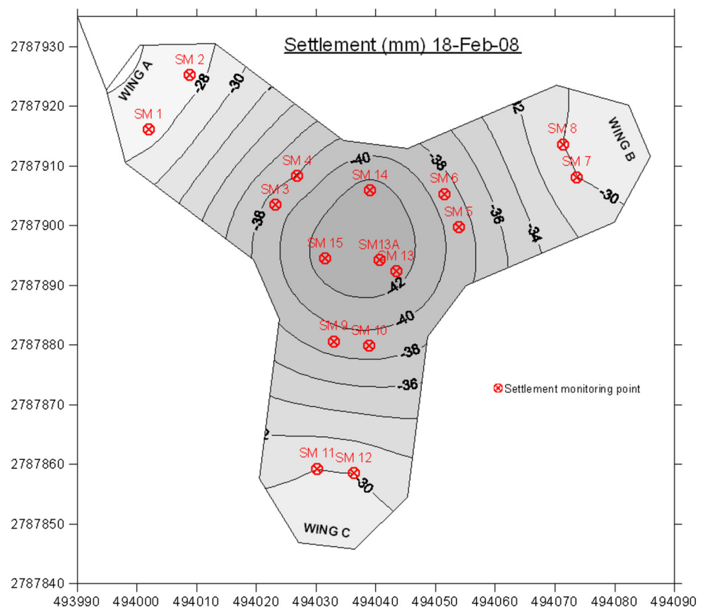
Fig. 18 Contours of measured settlement as at February 2008
